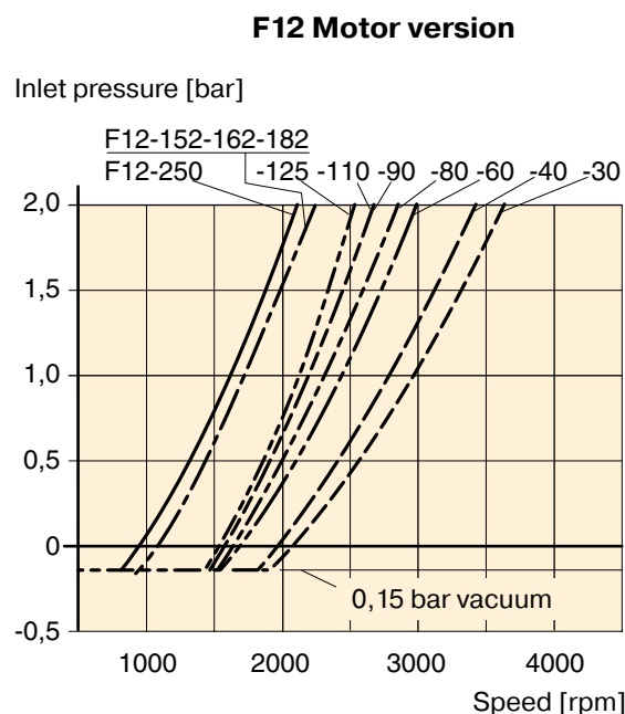
Diagram 3. Min. required motor (F12-M) inlet pressure.
