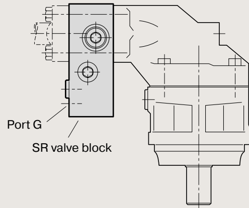
SR valve block location.
