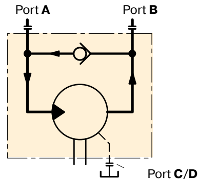
Schematic Fan motor with anti cavitation valve
